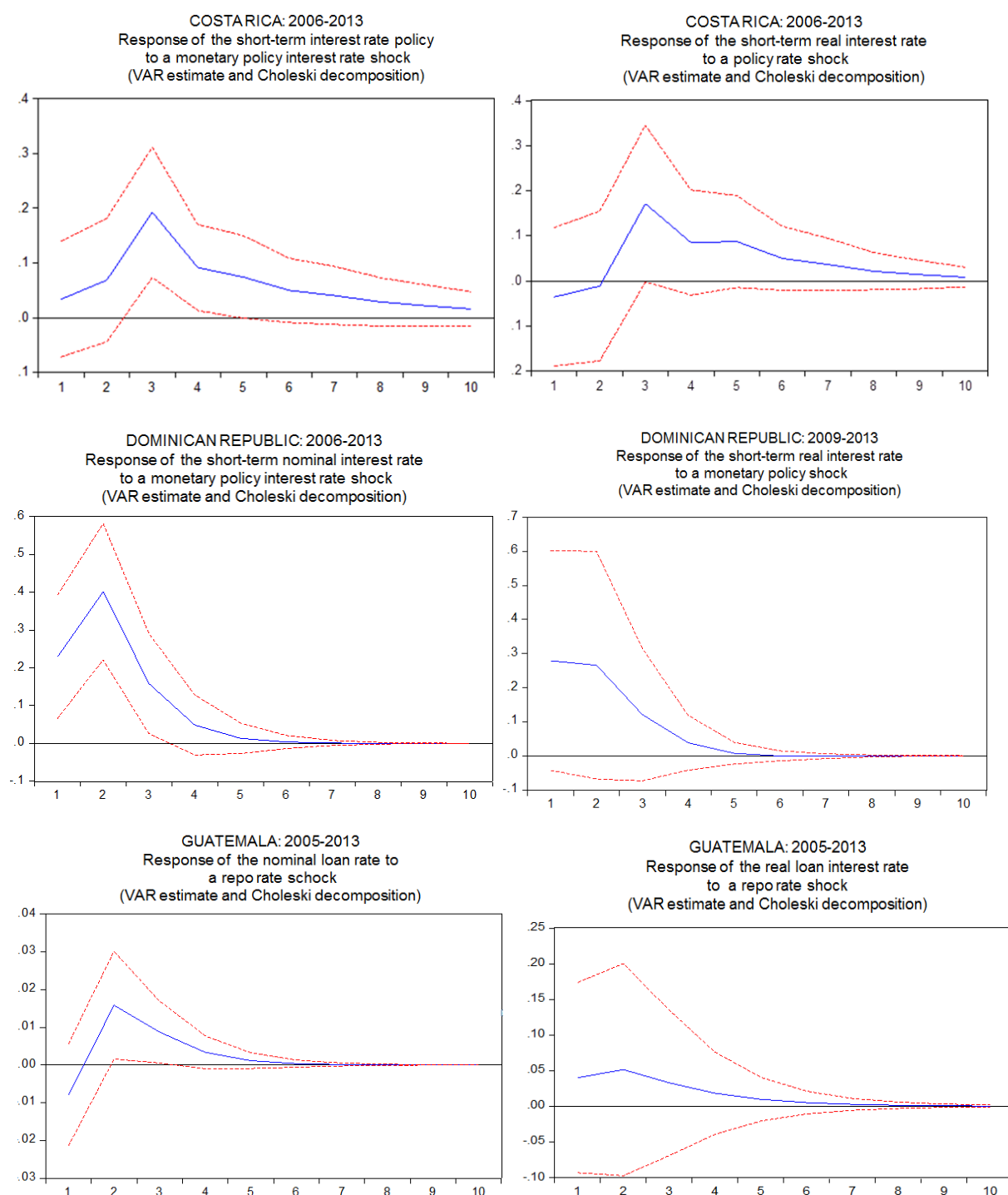
Figure 10. Impulse-Response Functions
